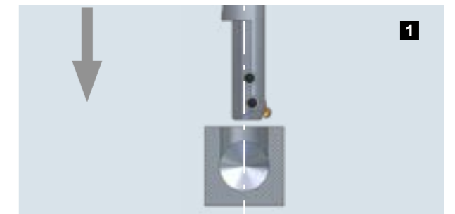
Approach with spindle stopped, orientated and offset 0
