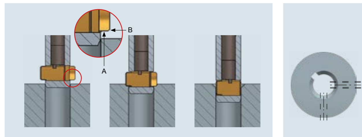
Fig. 1: Function principle DEFA tool
