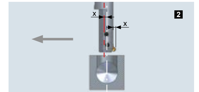
Approach offset dimension x. Value depends from the distance of the blade exceeding the tool body.
