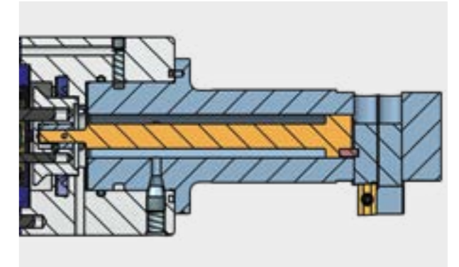
Image 2: SOLO2S Reinforced version
