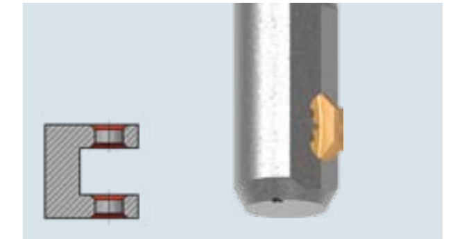
Chamfering front and back
